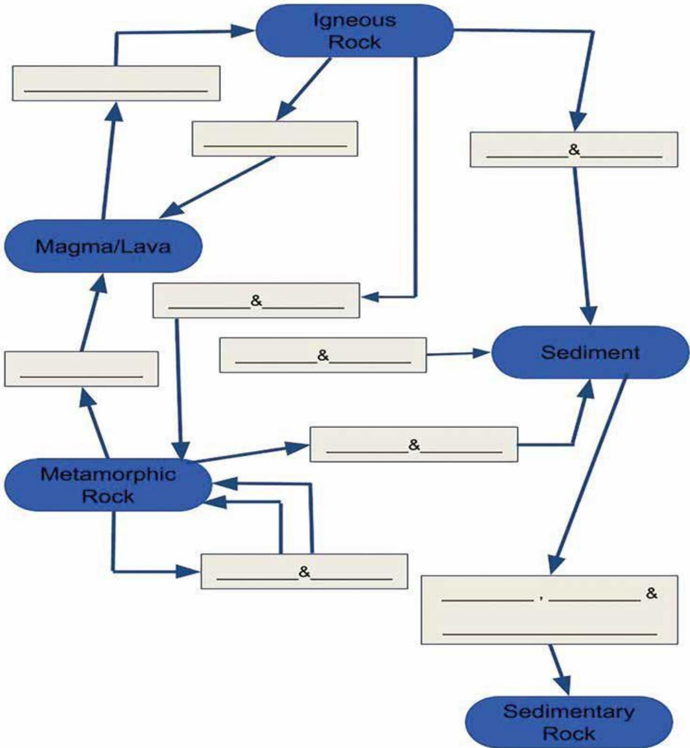
Rock Cycle Diagram
